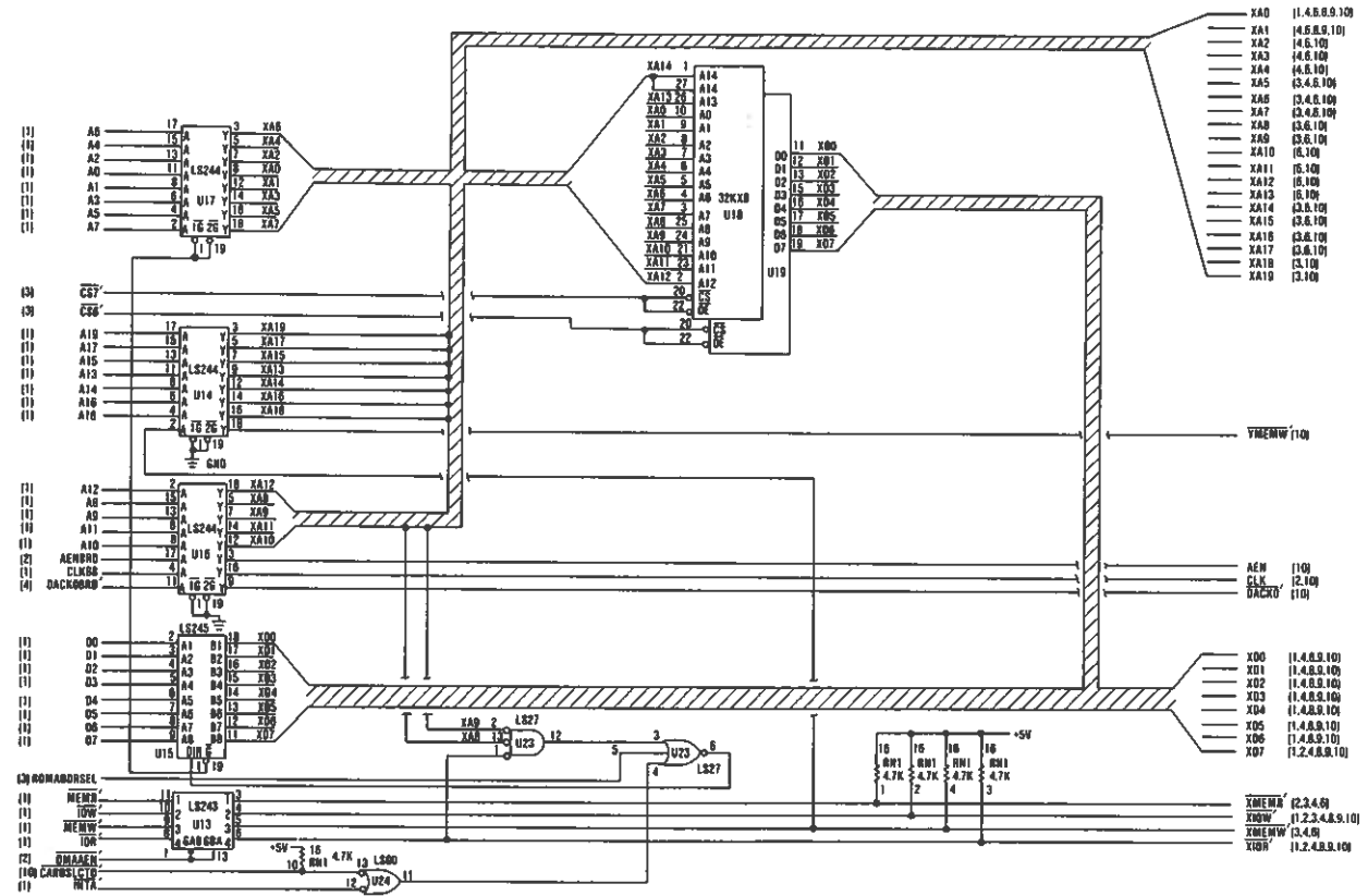
System Board (Sheet 5 of 10)
