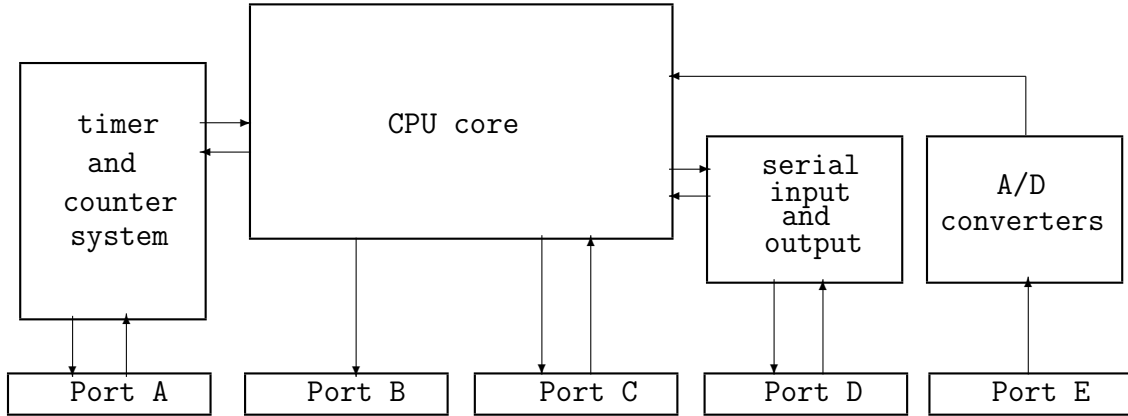
Figure 4: Simplified Block Diagram of HC11
