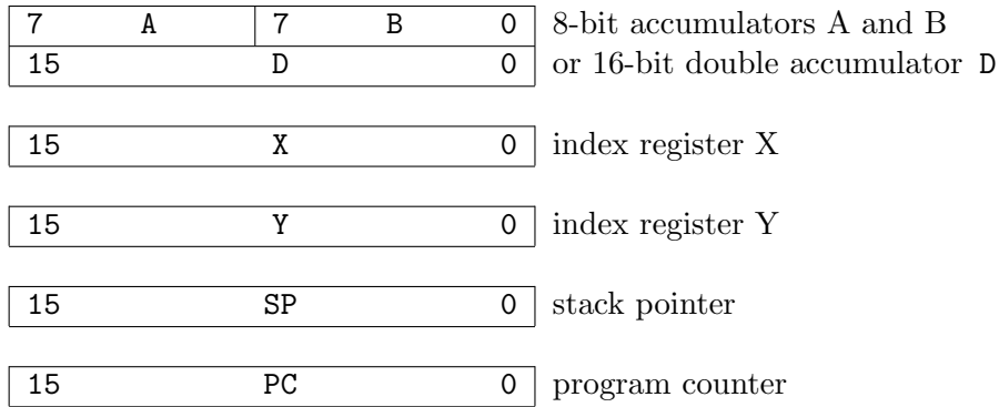
Figure 3: Programmer’s Model of HC11 Registers
