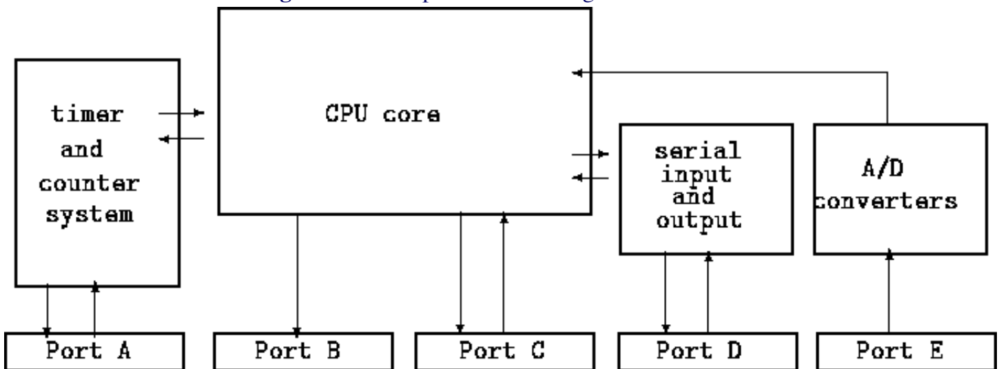
Figure 12.6: Simplified Block Diagram of 68HC11
